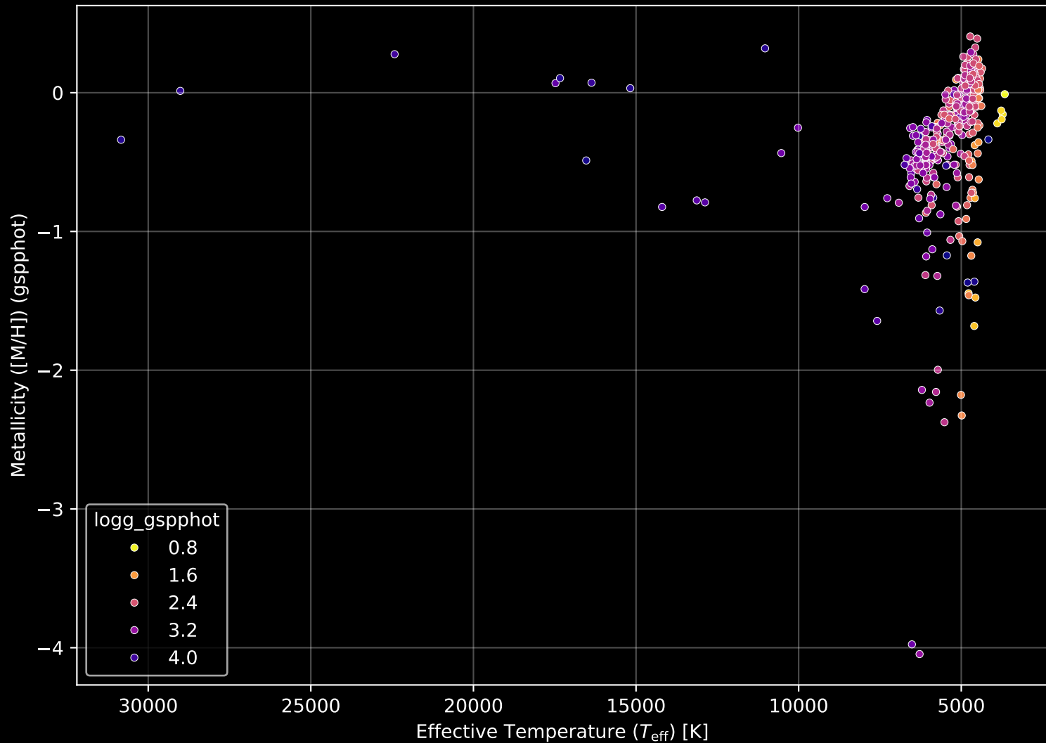
APOGEE DR17 Field: [010-07-C] Stellar Population Parameters (n= 430)
