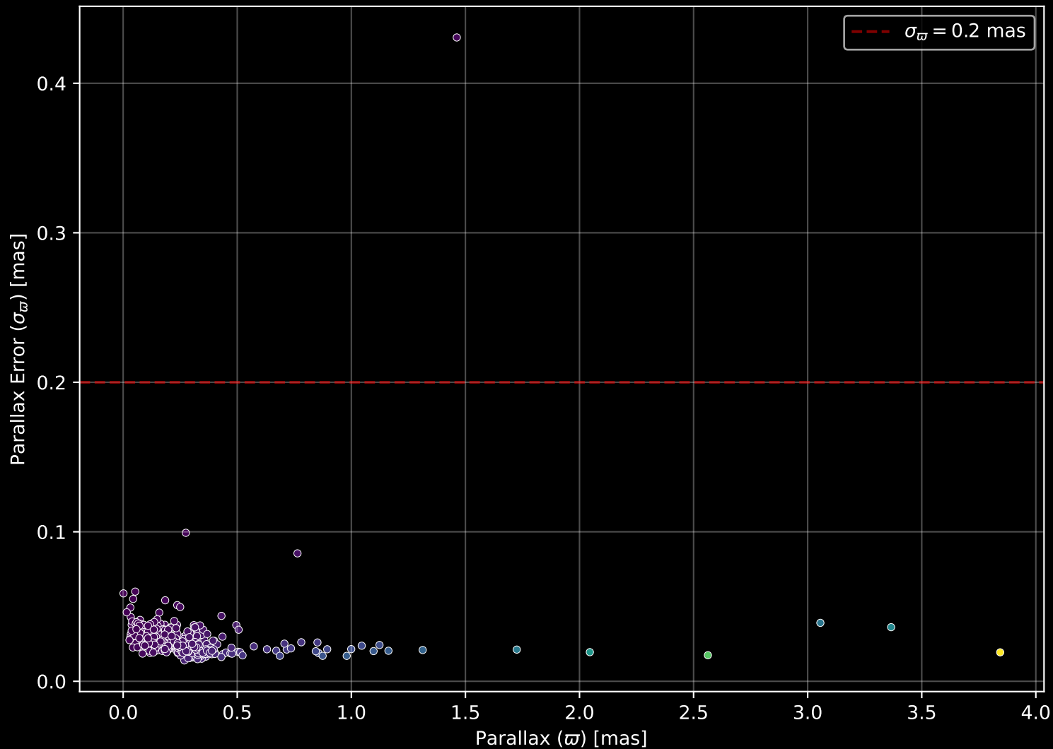
APOGEE DR17 Field: [010-07-C] Parallax Quality (n= 430)
