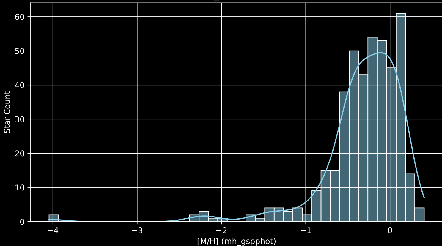
APOGEE DR17 Field: [010-07-C [M/H] (mh_gspphot) (n= 430)
