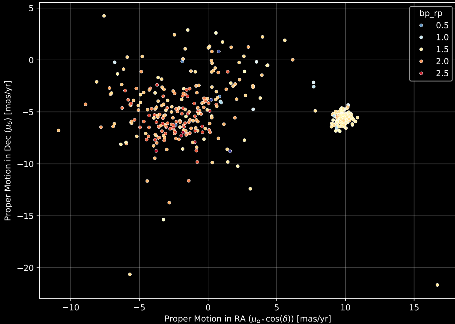
APOGEE DR17 Field: [010-07-C] Proper Motion Diagram (n= 430)
