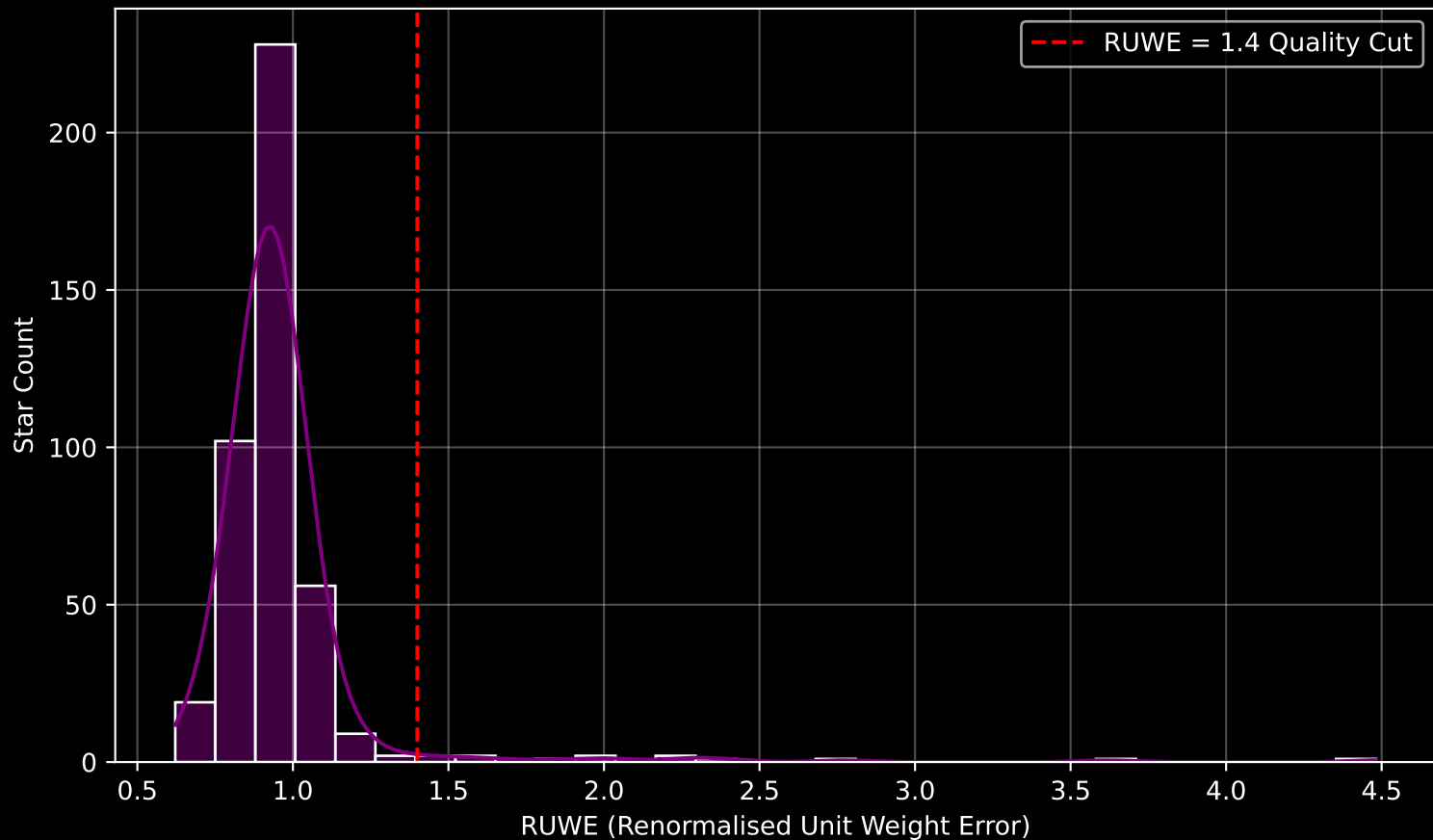
GAPOGEE DR17 Field [010-07-C] RUWE Distribution (n= 429)
