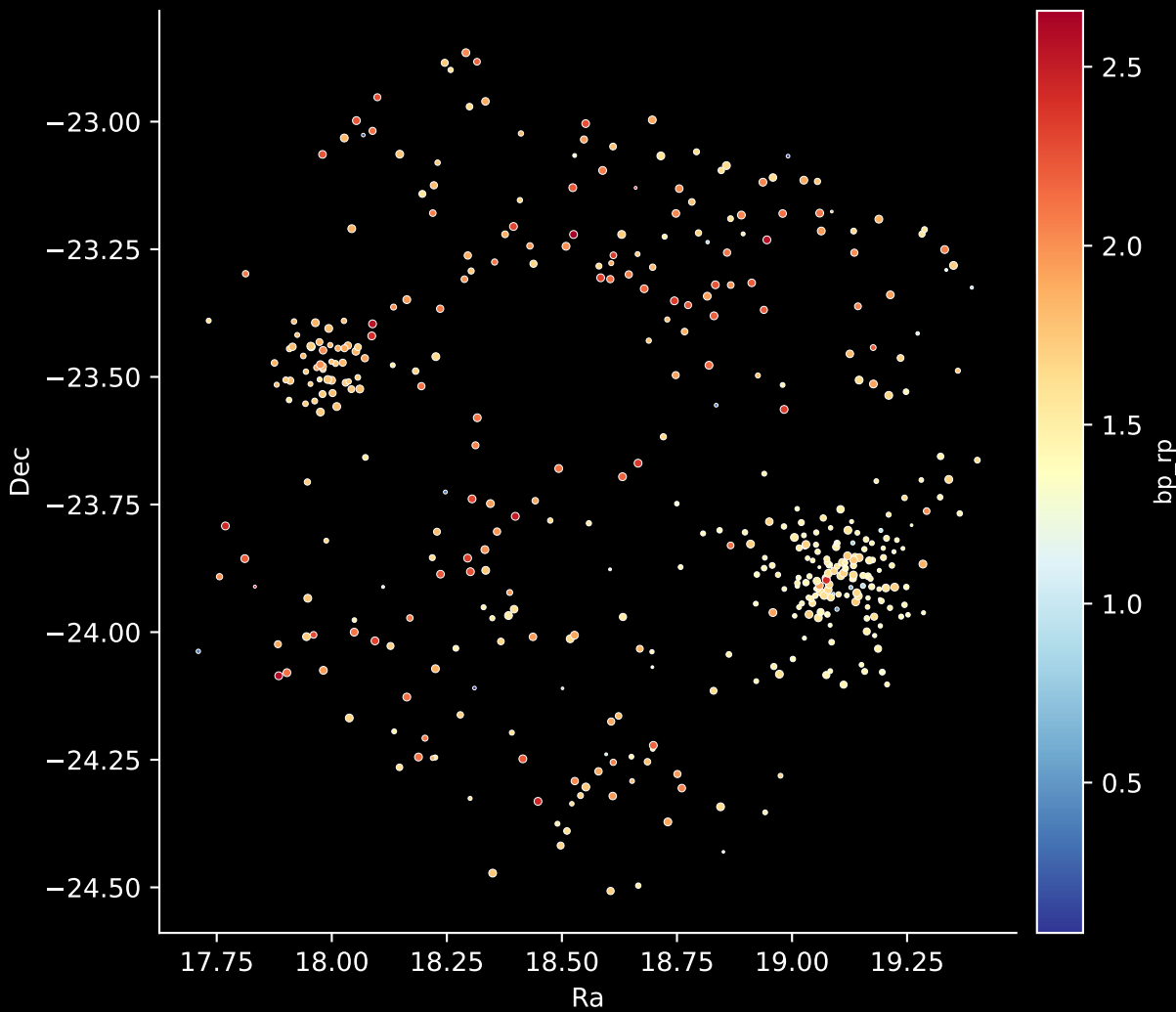
APOGEE DR17 Field: [010-07-C] Stars: 430
