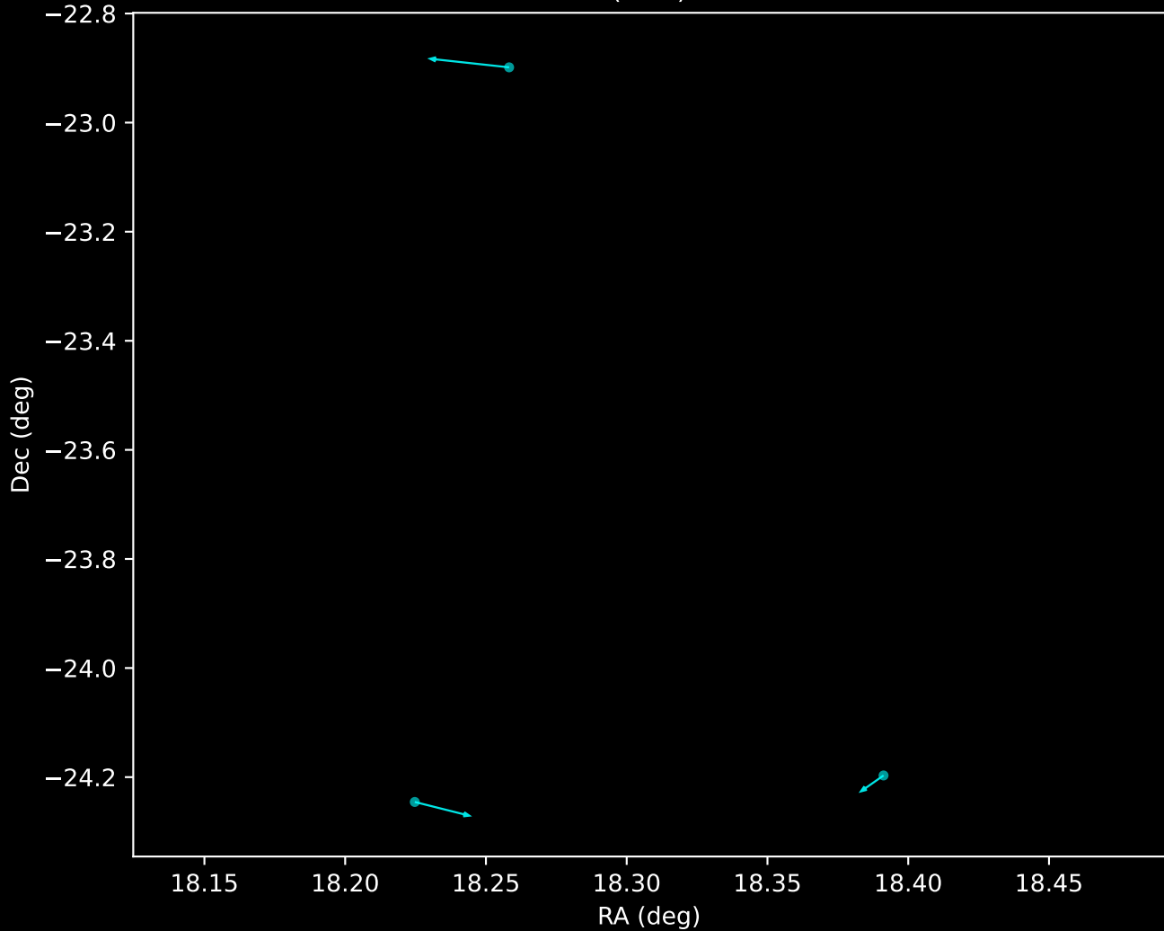
APOGEE DR17 Noise Stream Proper Motion Vectors (n=3)
