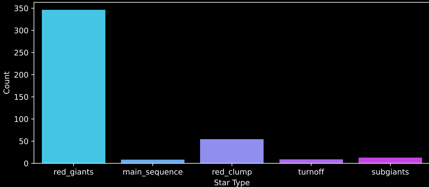
APOGEE DR17 Field: [010-07-C] Count plot of Star Type
